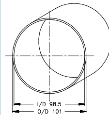
4" 16swg TUBE
